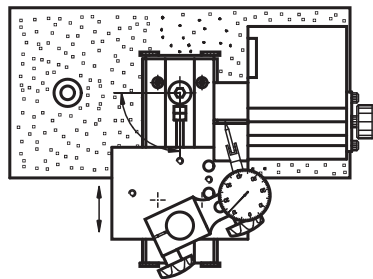
The slide can be rotated through 90° allowing rapid clearance and positioning for changing parts
