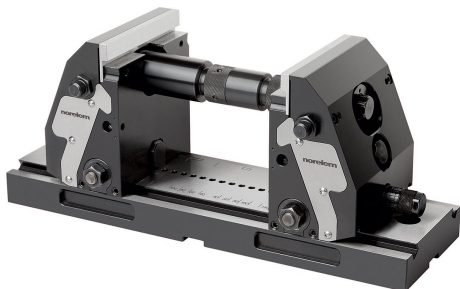
Tractive force 5-axis clamping system compact
