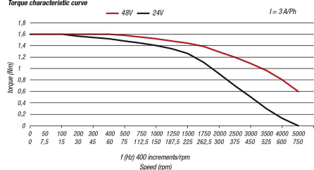
Torque characteristic curve
