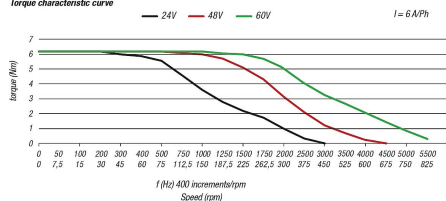
Torque characteristic curve
