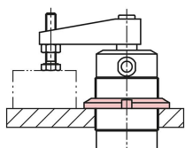
With a slotted round nut from above.
