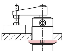
With a slotted round nut from below.
