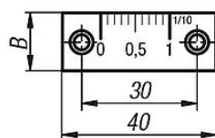
Vernier scale
