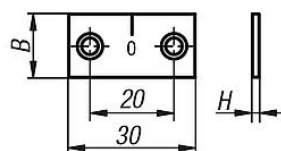
zero mark
