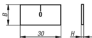
zero mark
