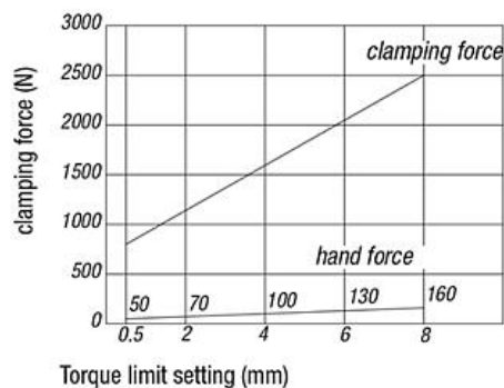
Pull Clamps 04400-4050...
