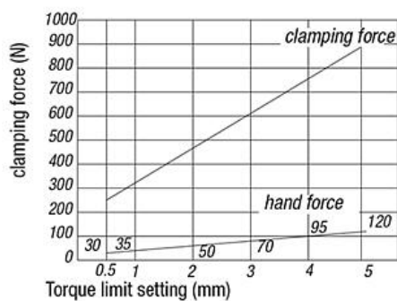
Pull Clamps 04400-3240...
