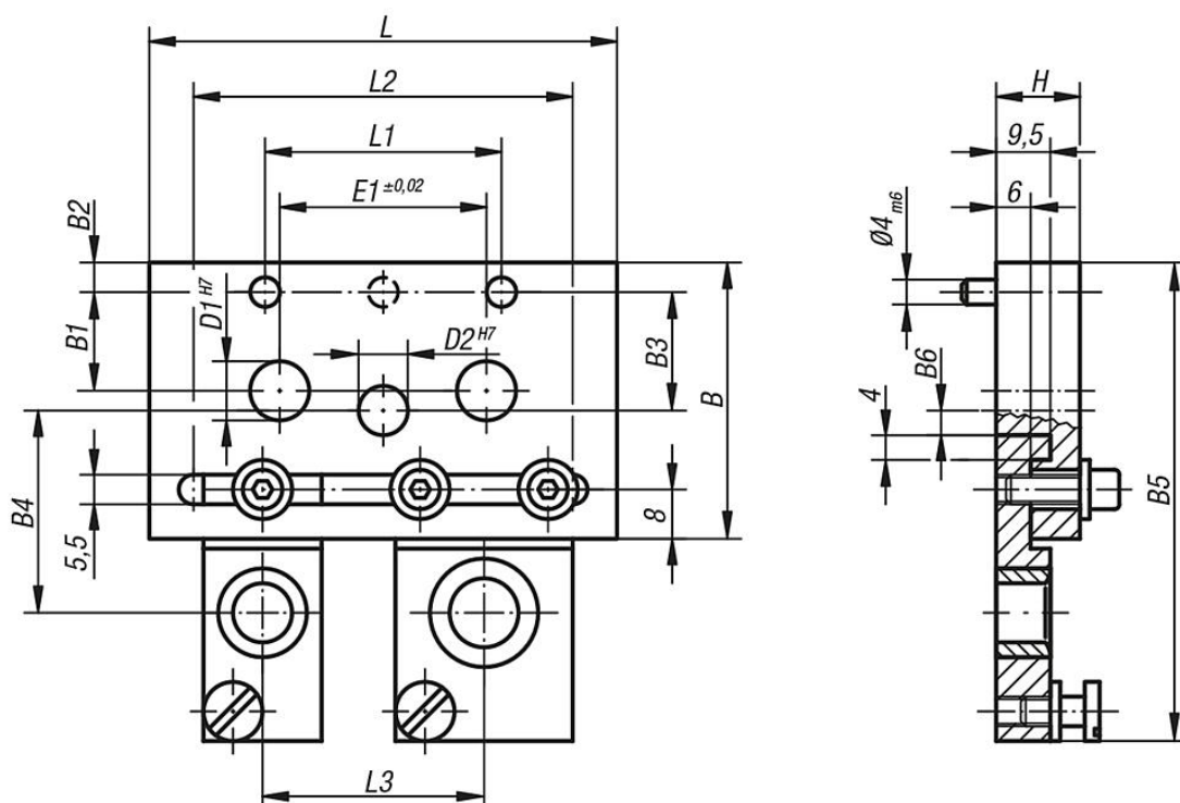
Drill bush holder plate
