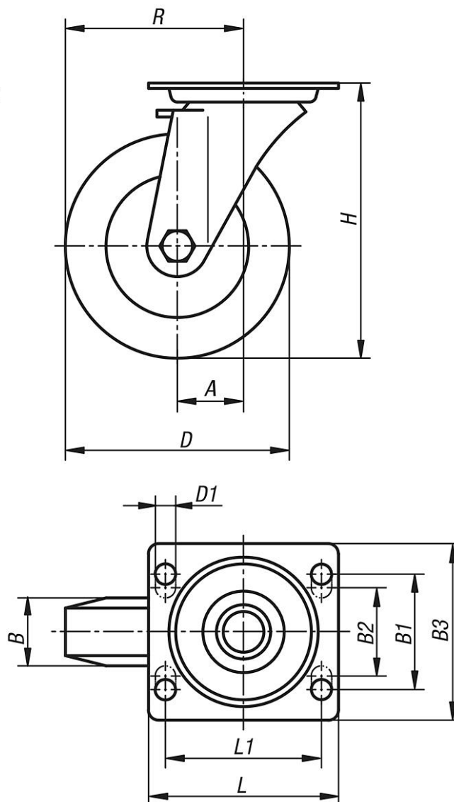
swivel castor
