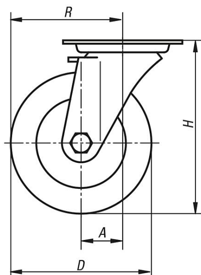
swivel castor
