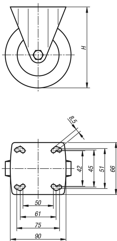
fixed castor
